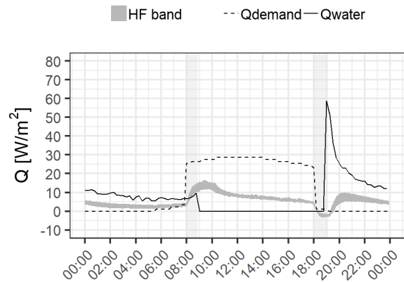
Fig. 9. Q_{water} , Q_{demand} and heat flux band.
