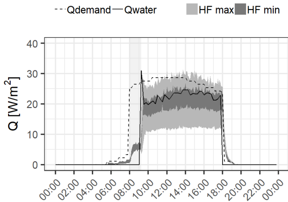
Fig. 5. Q_{\text{water}} , Q_{\text{demand}} and heat flux minimum and maximum band.
