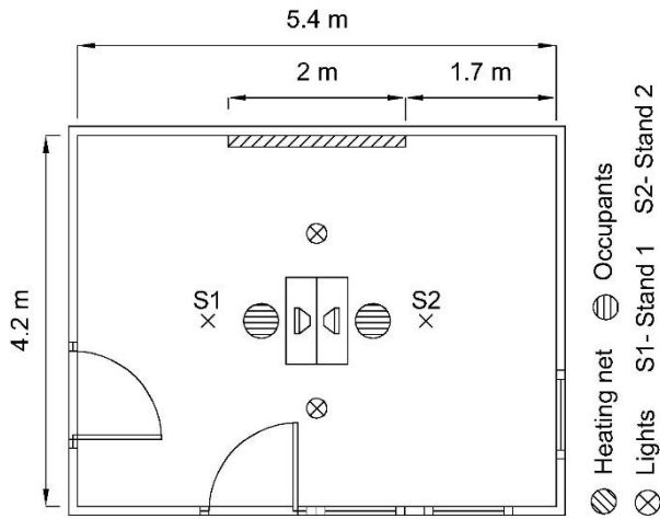
Fig. 2. Office room representation.
