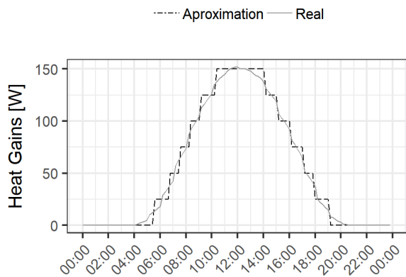
Fig. 3. Solar heat gains processing, SHG1.
