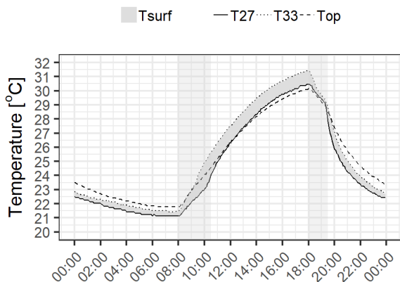
Fig. 11. Surface temperature of panels measured by PT1000 sensors PCM D.
