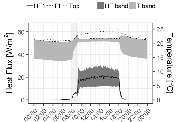
Fig. 6. Heat flux, surface temperatures and operative temperature RCP A.
