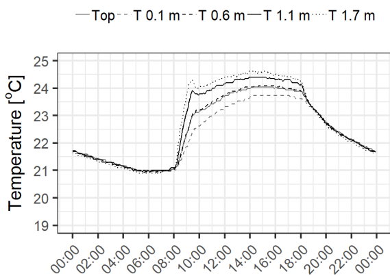
Fig. 8. Average temperatures measured on the stands for RCP A.
