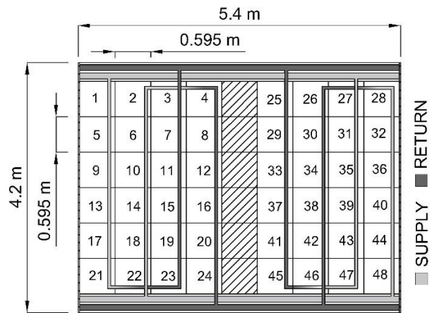
Fig. 4. Pipe network.
