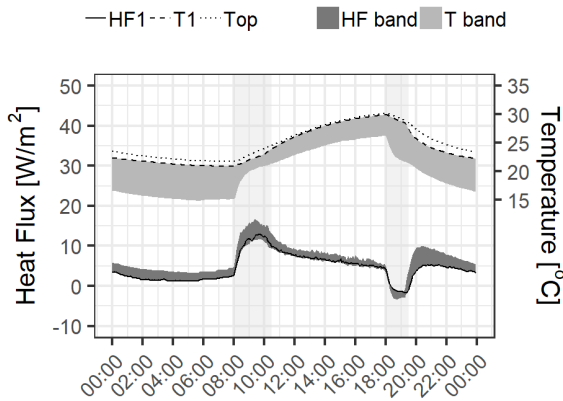
Fig. 10. Heat flux and surface temperatures and operative temperature PCM D.
