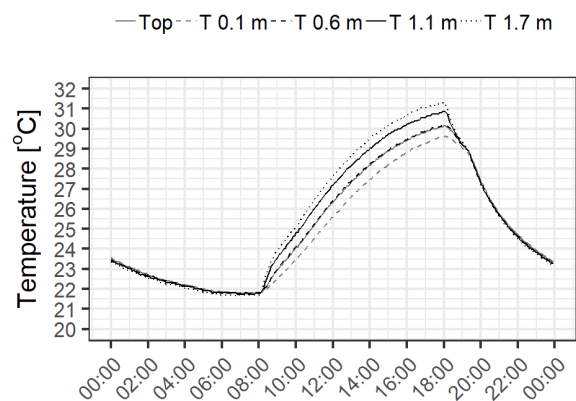
Fig. 12. Average temperatures measured on the stands for PCM D.
