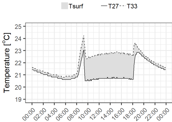
Fig. 7. Surface temperature of panels measured by PT1000 sensors RCP A.
